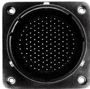
MIL-C-38999, SERIES 1, BAYONET COUPLING
